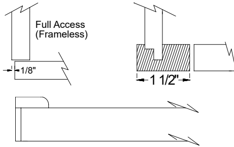
Section view of door style
