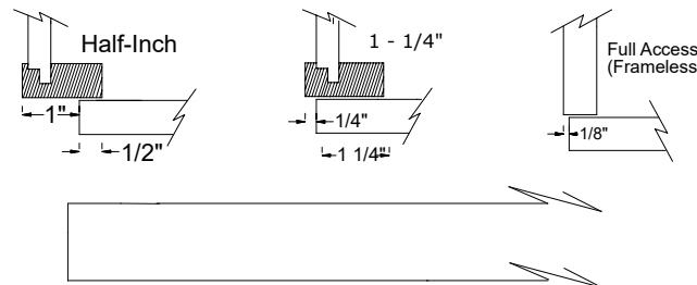
Section view of door style
